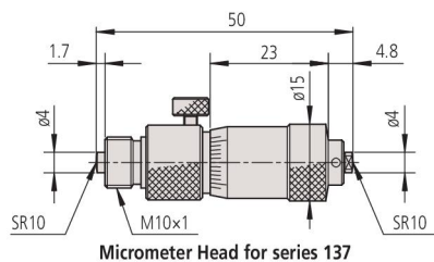
Micrometer Head for series 137
