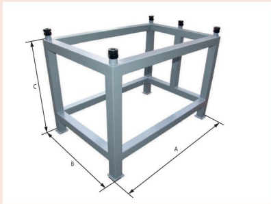
Dimensions for stand
