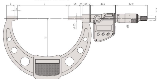
Ratchet stop type over 100 mm
