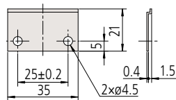
Retaining spring A
