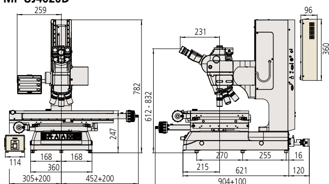
MF-UJ4020D
