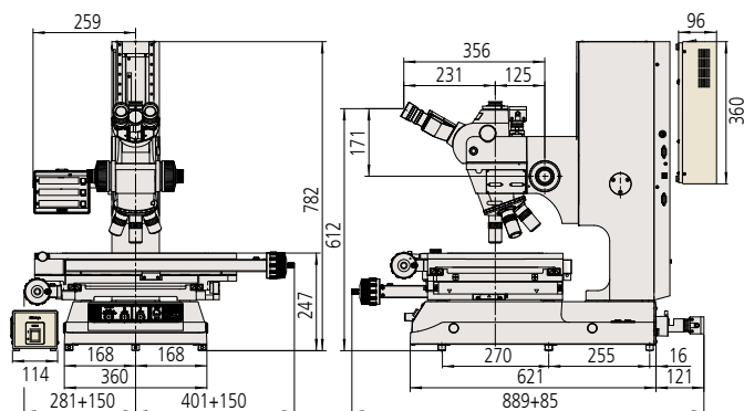
MF-UB3017D
