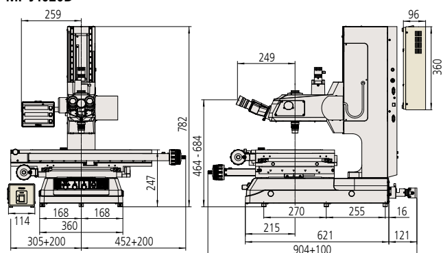
MF-J4020D
