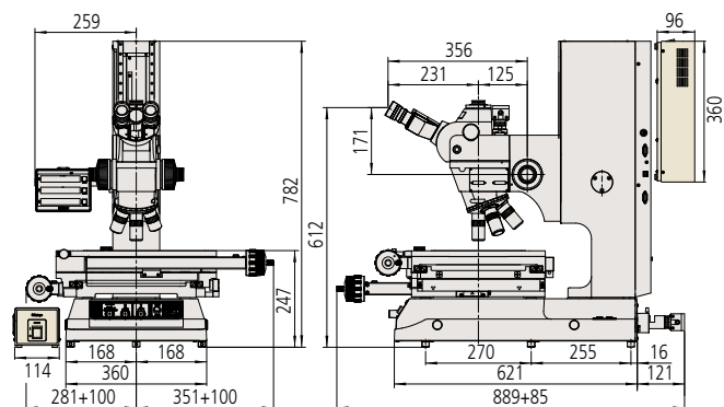
MF-UB2017D
