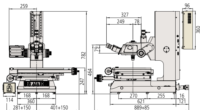
MF-B3017D
